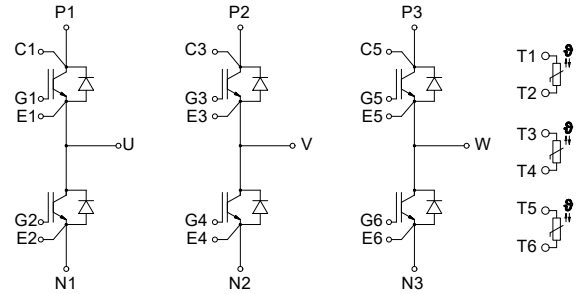
等效电路图 Equivalent Circuit Schematic
